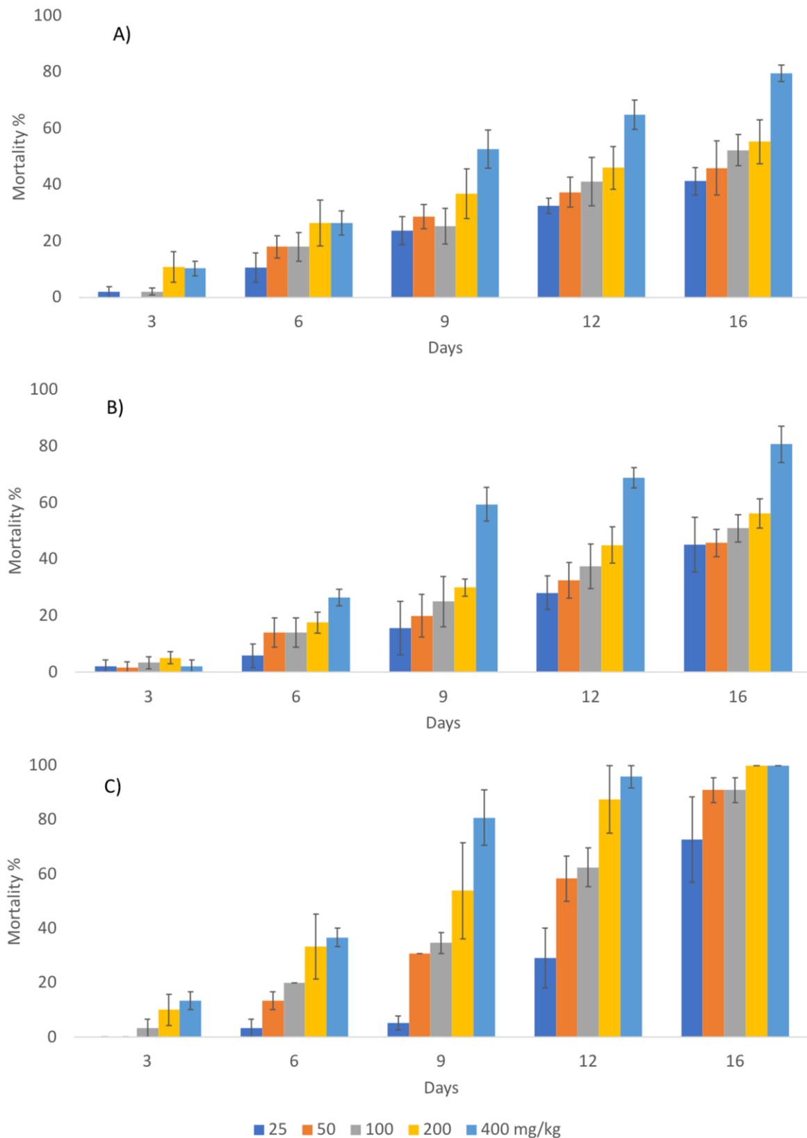
Figure 3. Mortality (%) (mean \pm SE) of T. confusum (a) and O. surinamensis (b) S. paniceum (c) adults fed on beans treated with nanostructured alumina (NSA) particles.
