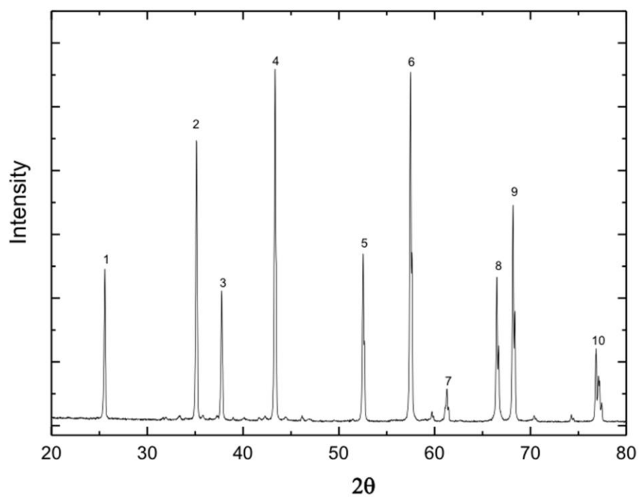
Figure 1. X-ray diffraction (XRD) spectra of the nanostructured alumina (NSA) particles
